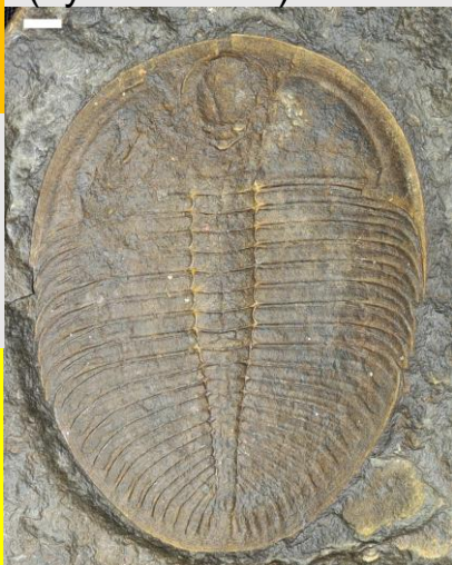
Ogygiocaris (hyd at 12cm)
