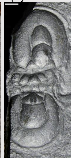
Geragnostus (hyd at 1cm)
